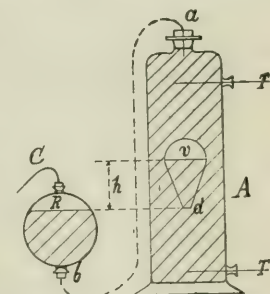
FIG. 1.—Cartesian diver adjusted for diffusion measurement.
